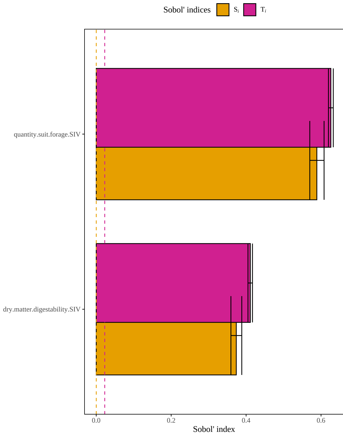
Figure 5. Results of a sensitivity analysis for the whitetaileddeerModelII model based on a geometric mean structure. Dashed lines represent baseline numerical approximation error for S_i and T_i ( i.e. , dummy variables).
