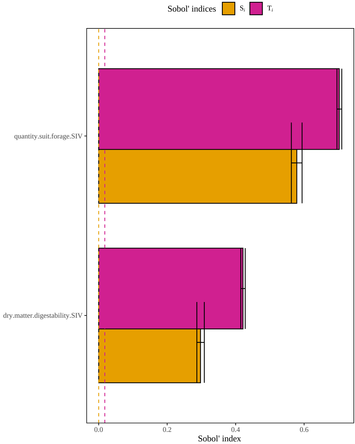
Figure 6. Results of a sensitivity analysis for the whitetaileddeerModelIII model based on a limiting factor structure. Dashed lines represent baseline numerical approximation error for S_i and T_i ( i.e. , dummy variables).
